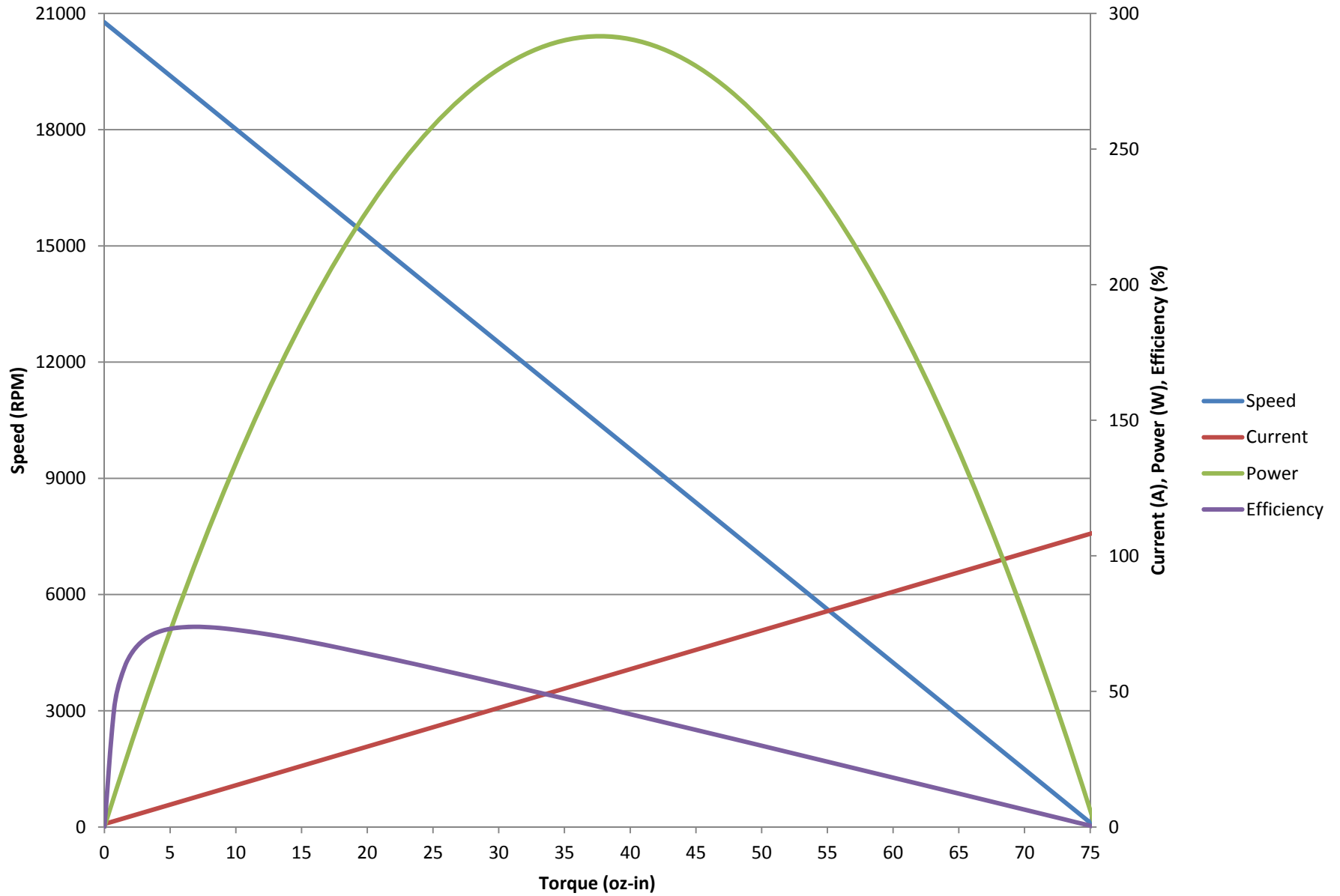
Fisher-Price (-0673) Motor Curve
